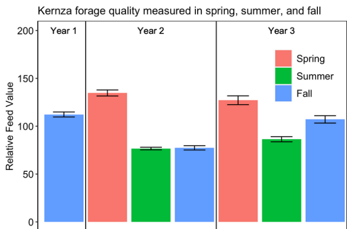
Fig. 3. Kernza Forage Quality, Years 1 - 3
