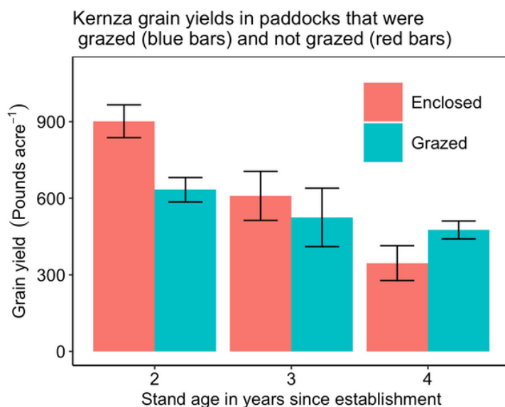
Fig. 1 Kernza Grain Yield, Years 2 - 4
