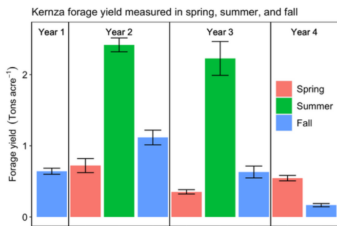
Fig. 2. Kernza Forage Yield, Years 1 - 4
